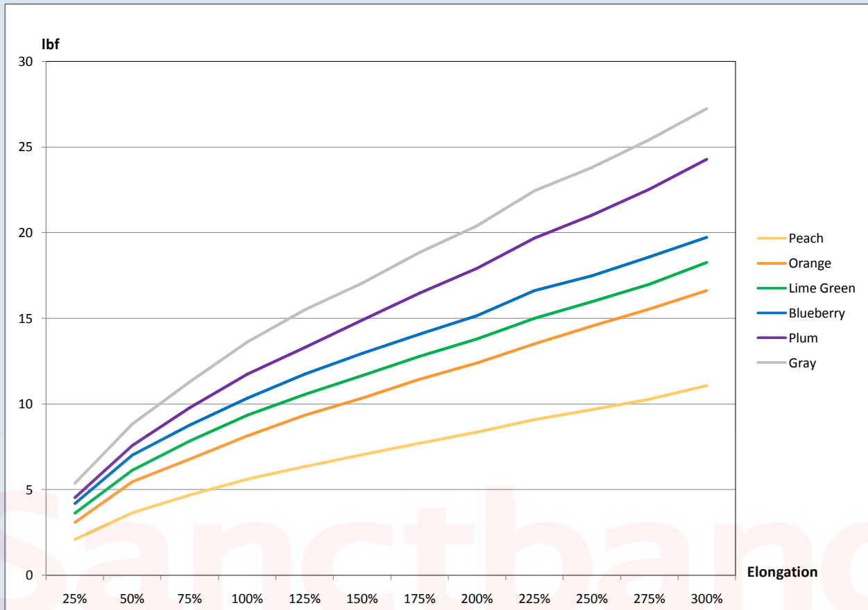
Figure: Force-Elongation of Sanctband Exercise Tubing - ID 6.5mm
