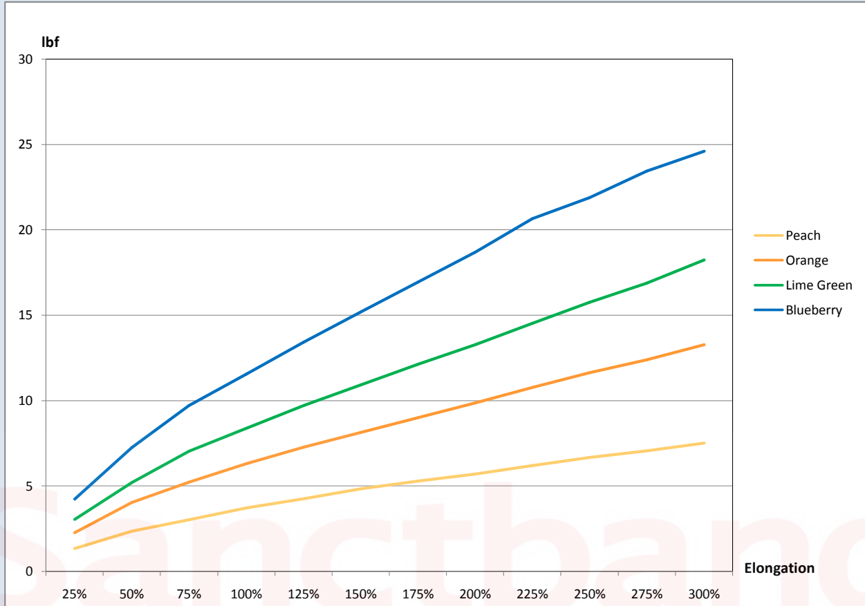
Figure: Force-Elongation of Sanctband Loop Bands
